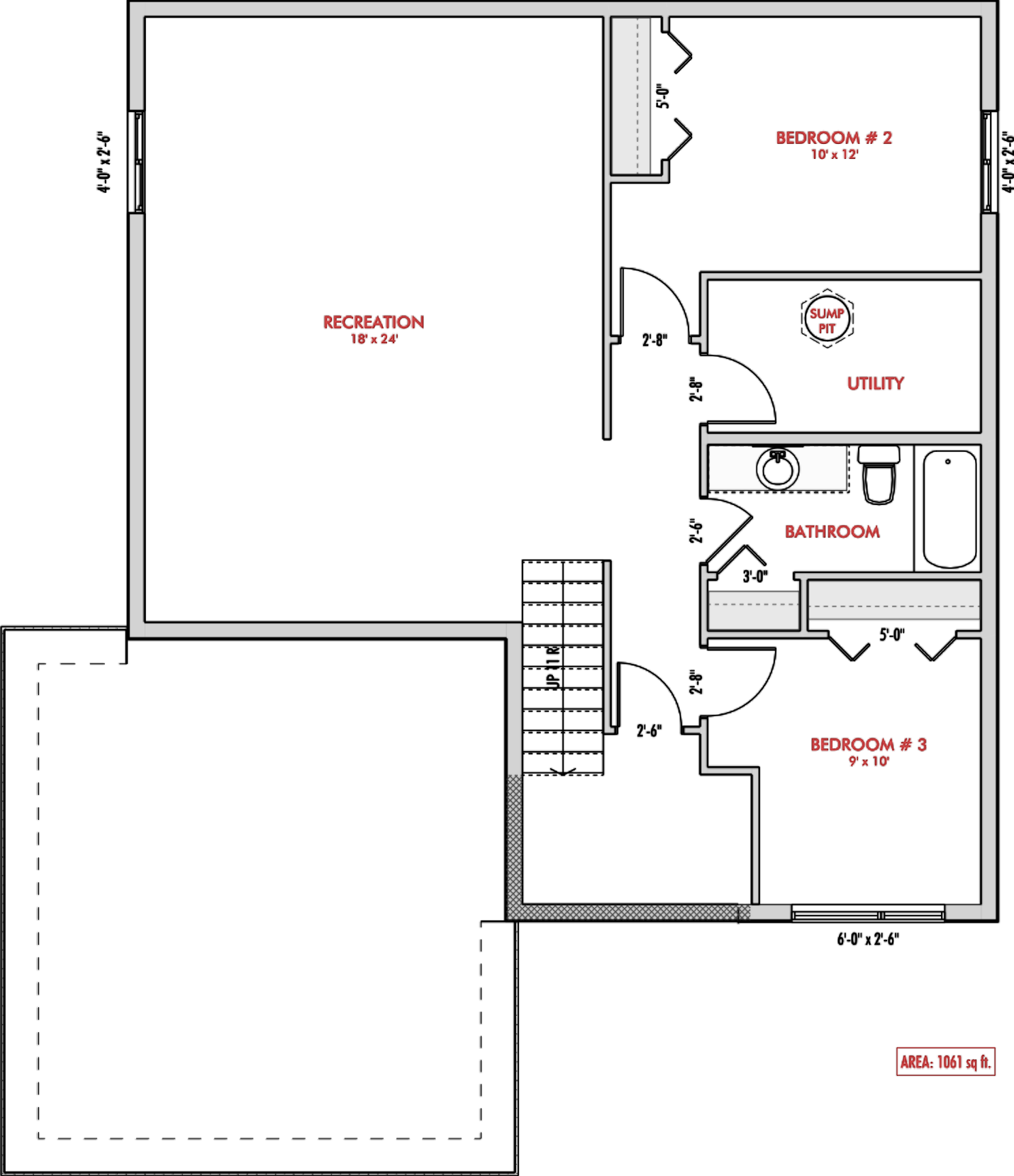
BASEMENT PLAN
