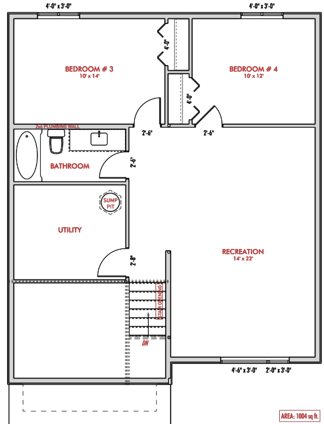
BASEMENT PLAN
