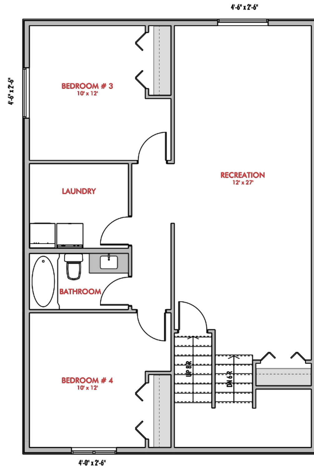
BASEMENT PLAN
