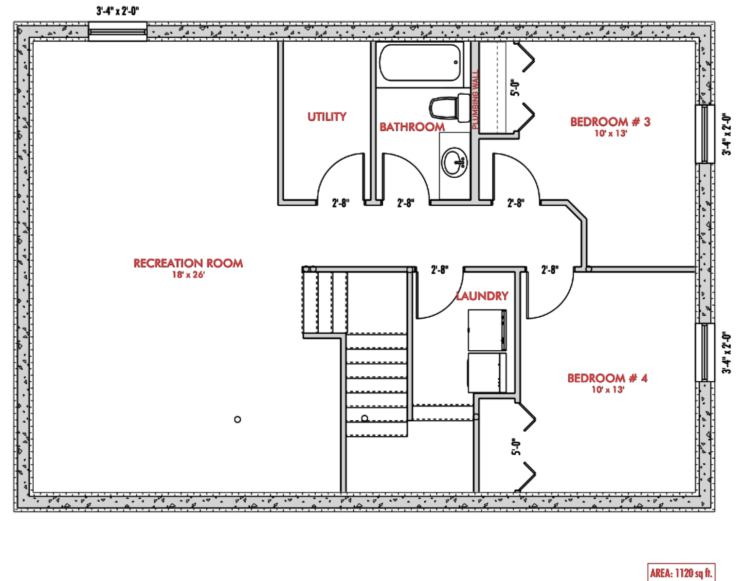
BASEMENT LAYOUT
